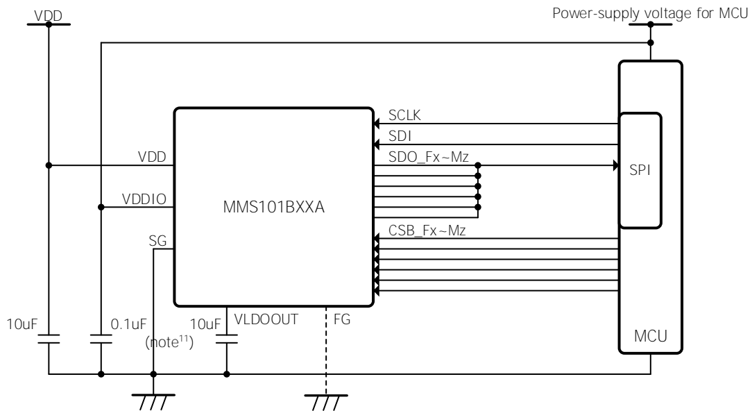
Fig. 25 Integrated SDO pin – Example application circuit
