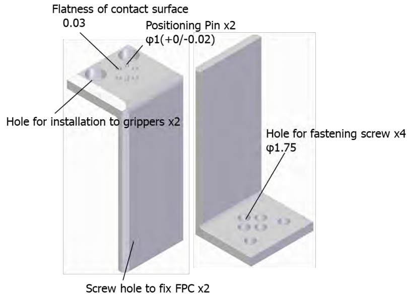
Fig. 30 Example of bottom side attachment
