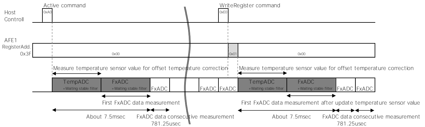
Fig. 15 Schematic of update of temperature sensor values for offset temperature correction
