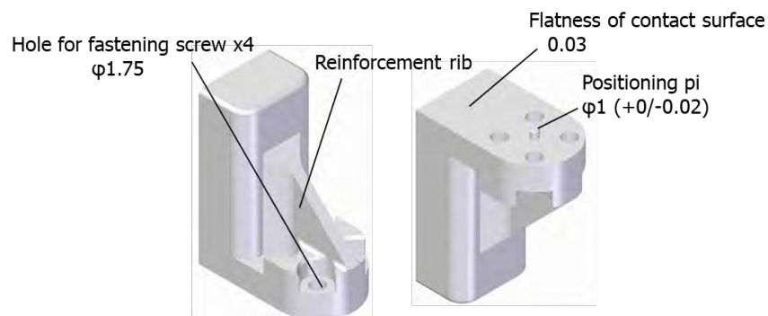
Fig. 29 Example of top side attachment
