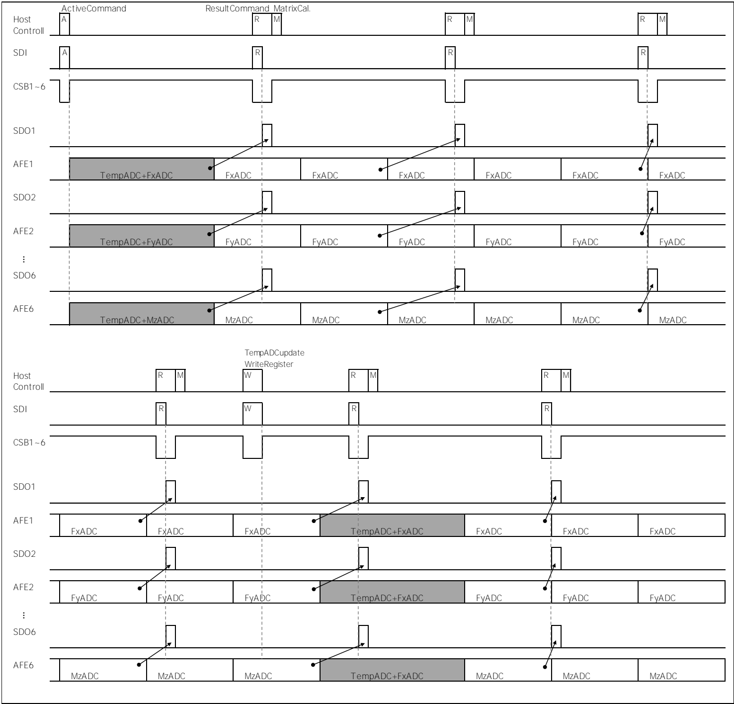
Fig. 16 Integrated CSB pin - Measurement timing chart
