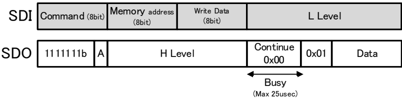
Fig. 22 SPI Write/Read format (Busy)
