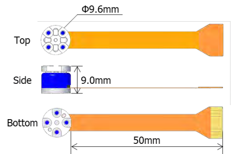
Fig. 1 Product appearance
