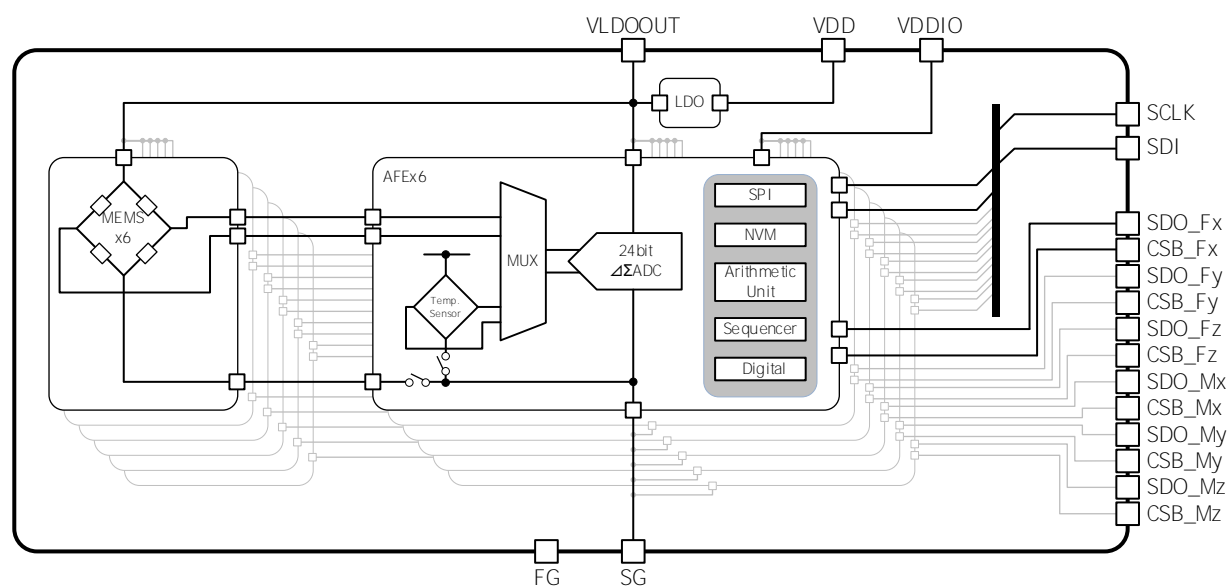
Fig. 2 Block Diagram
