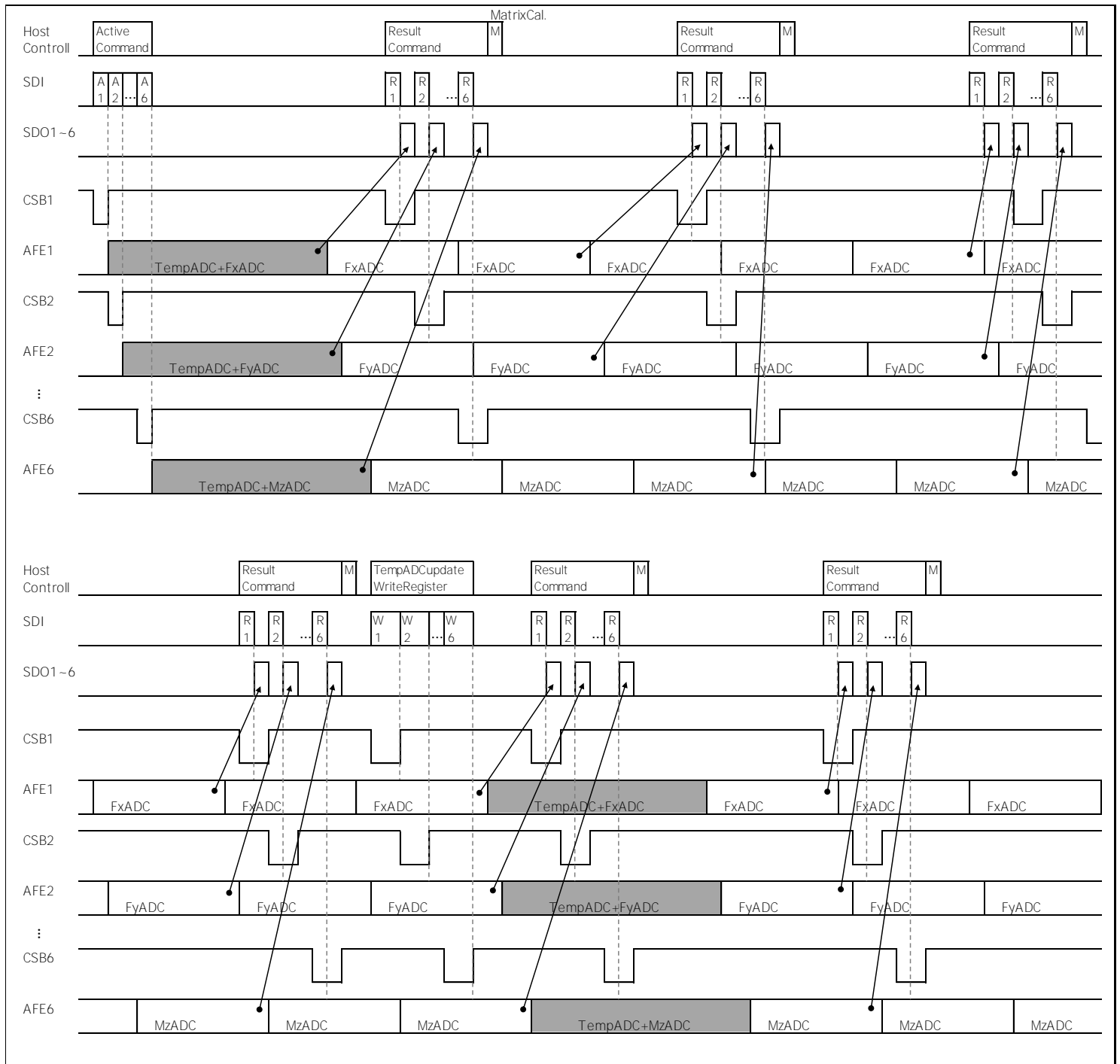
Fig. 17 Integrated SDO pin - Measurement timing chart
