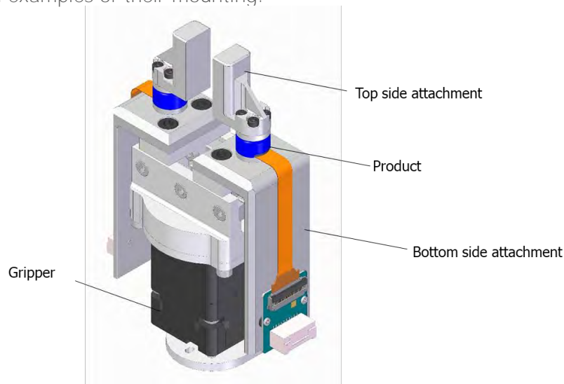
Fig. 28 Gripper-mounted image
