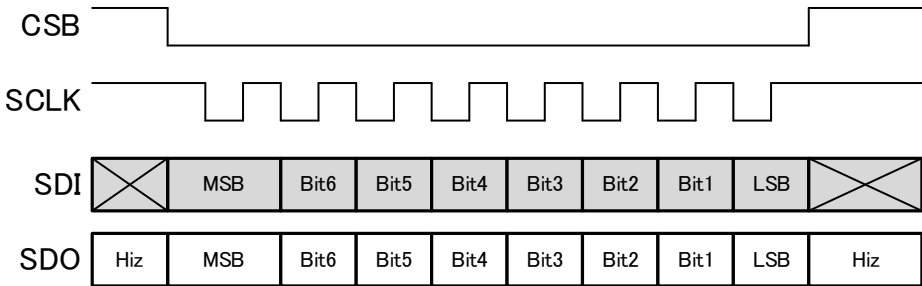
Fig. 19 SPI Waveform
