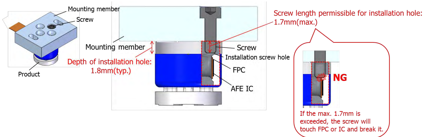
Fig. 33 Precautions for installation screw
