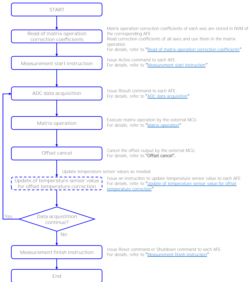
Fig. 9 Operation flow chart
