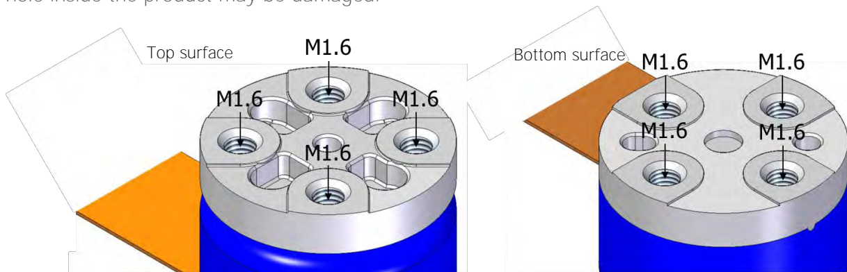
Fig. 32 Installation screw hole
