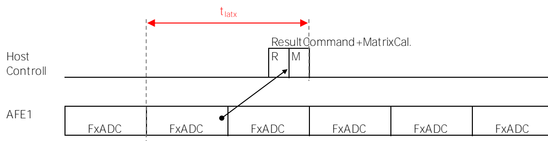
Fig. 8 Latency (e.g.: Fx)
