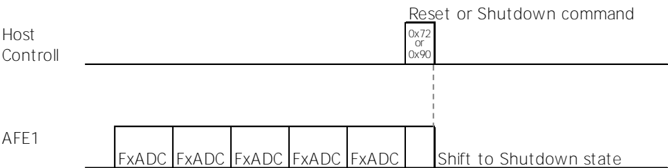
Fig. 14 Schematic of measurement finish instruction
