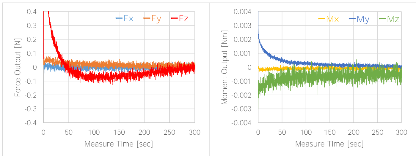
Fig. 12 Outputting data immediately after AD conversion starts
