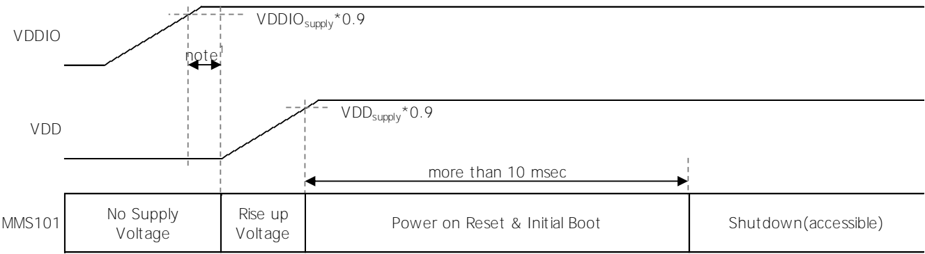
Fig. 4 Power-on sequence
