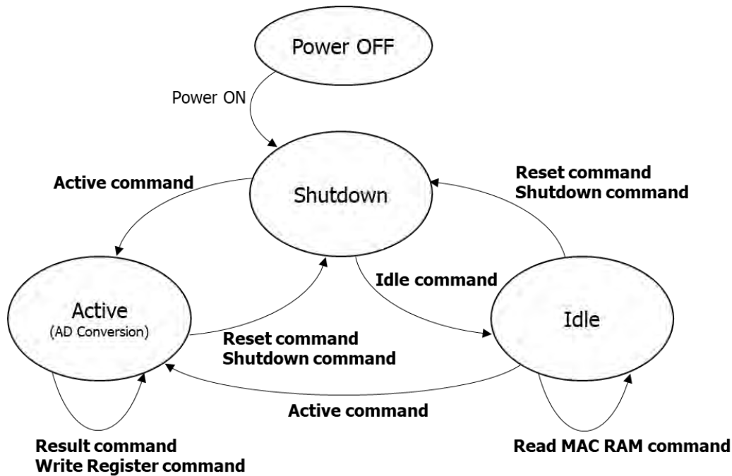
Fig. 18 State transition diagram
