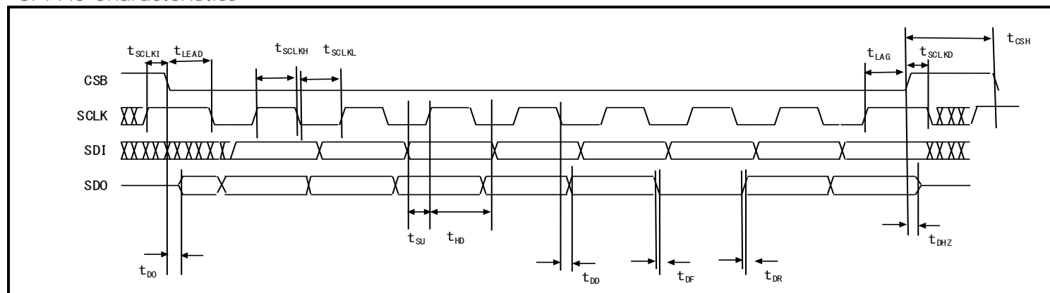
Fig. 23 SPI AC timing chart
