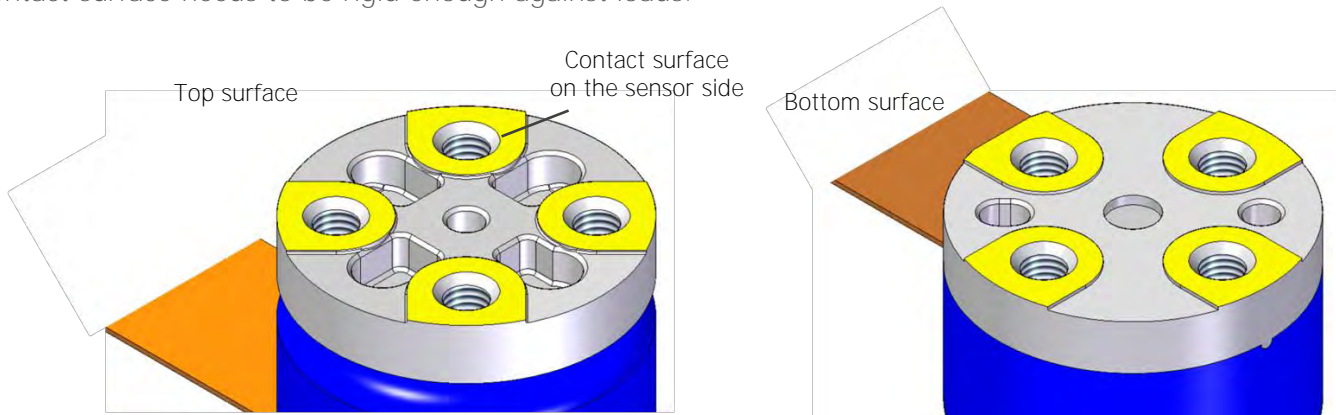
Fig. 36 Sensor side contact surface
