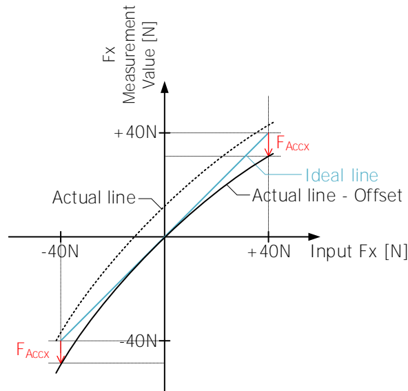
Fig. 7 Accuracy (e.g.: Fx)
