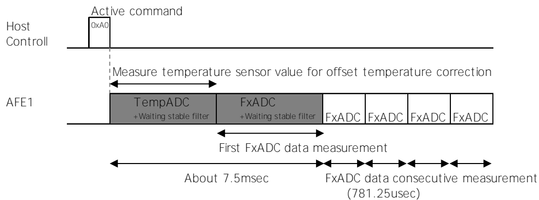
Fig. 11 Schematic of AD conversion start instruction
