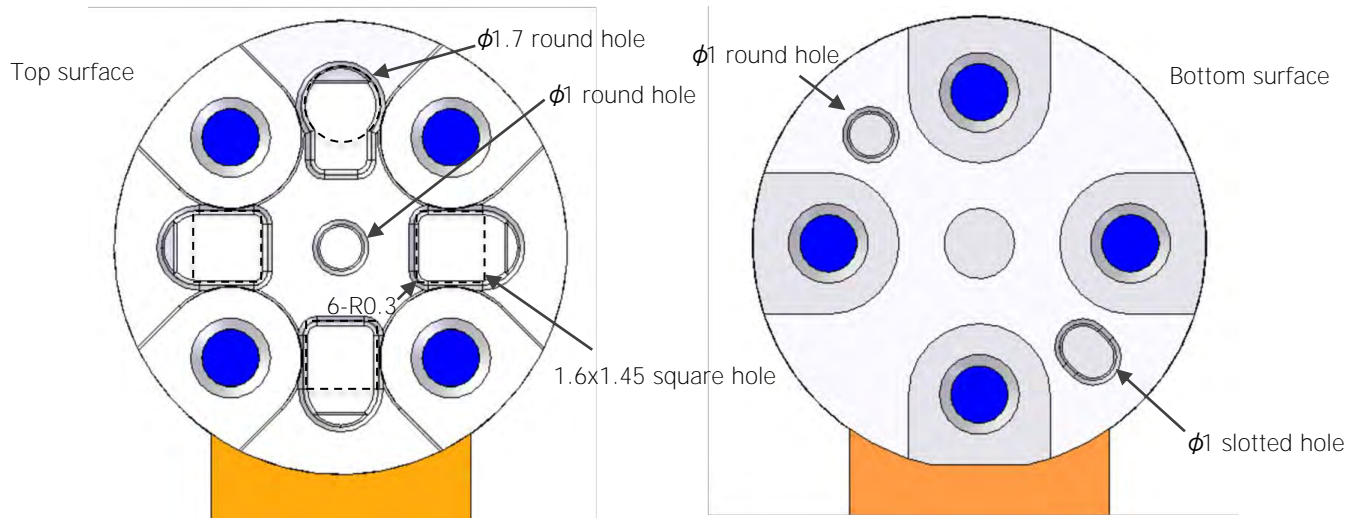
Fig. 34 Positioning holes
