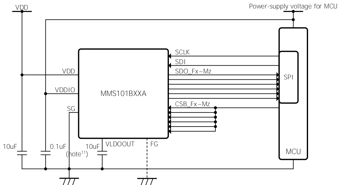
Fig. 24 Integrated CSB pin – Example application circuit
