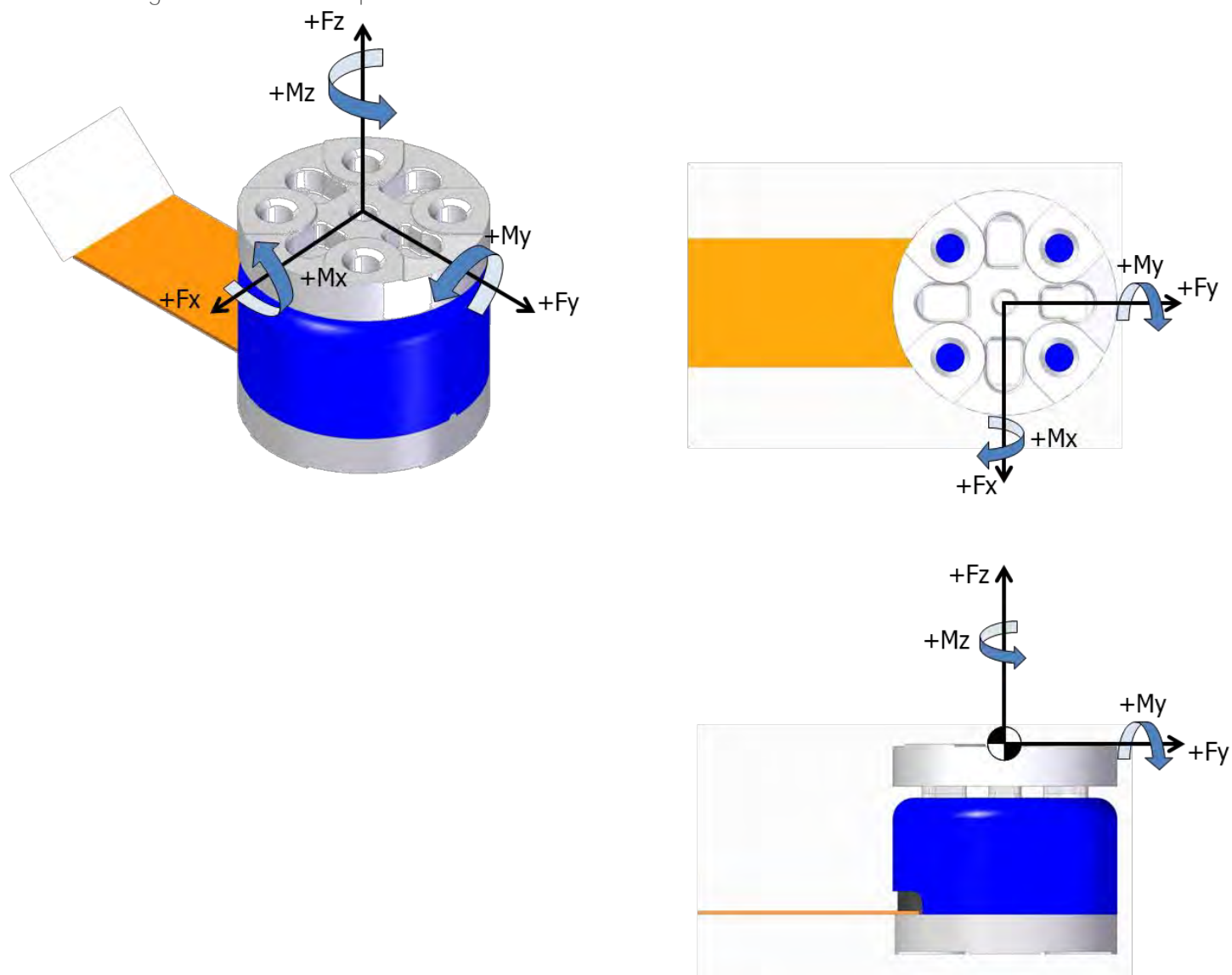
Fig. 27 Sensor coordination systems
