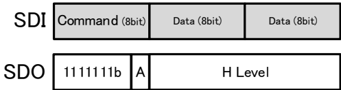
Fig. 20 SPI Write format
