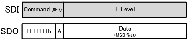
Fig. 21 SPI Write/Read format
