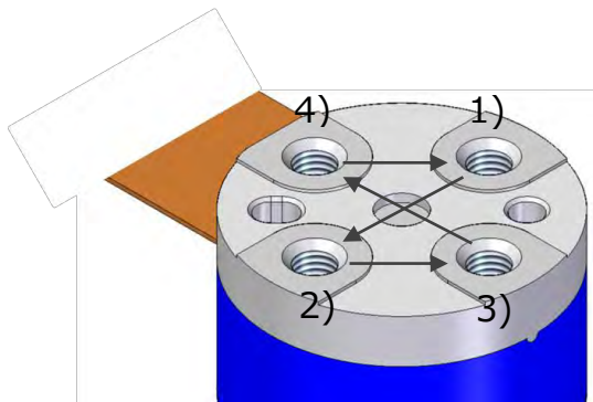
Fig. 35 Example of screw tightening order
