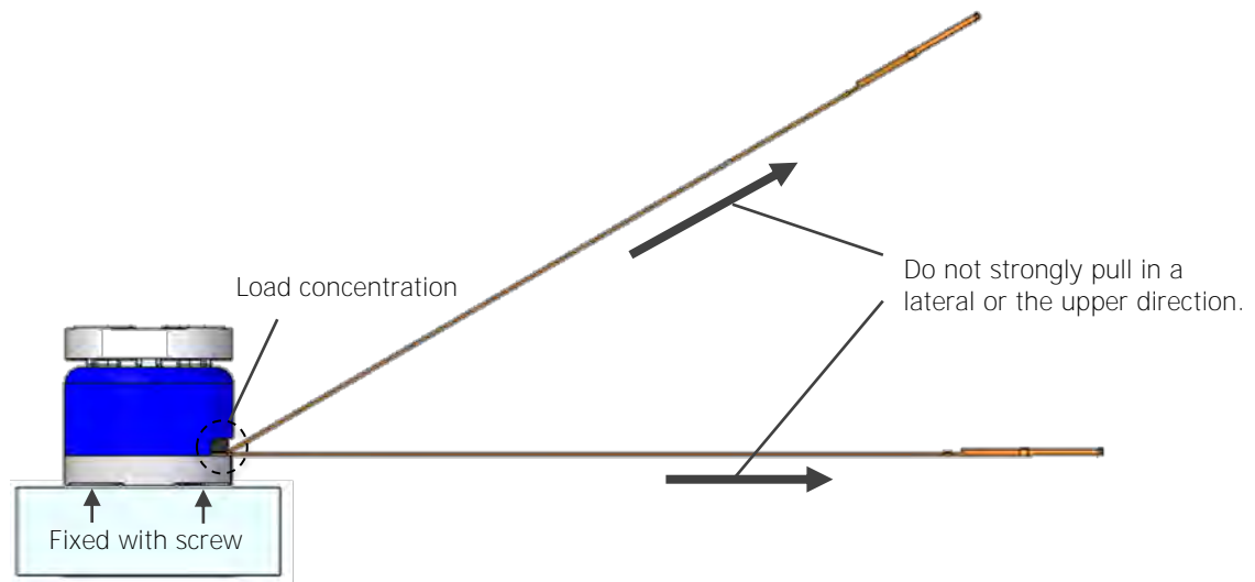
Fig. 37 Precaution for handling of sensor FPC - 1
