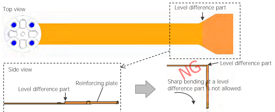
Fig. 38 Precaution for handling of sensor FPC - 2
