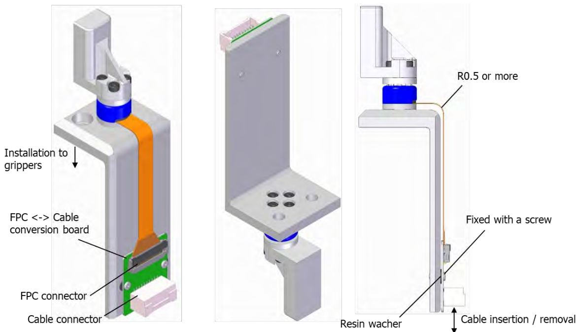
Fig. 31 Example of attachment installation
