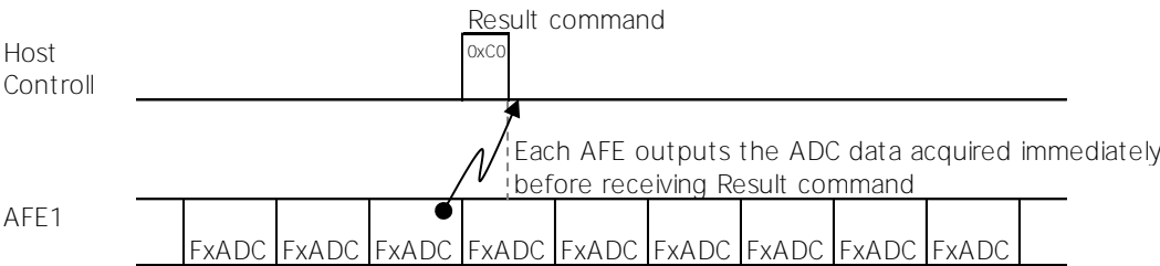
Fig. 13 Schematic of ADC data acquisition
